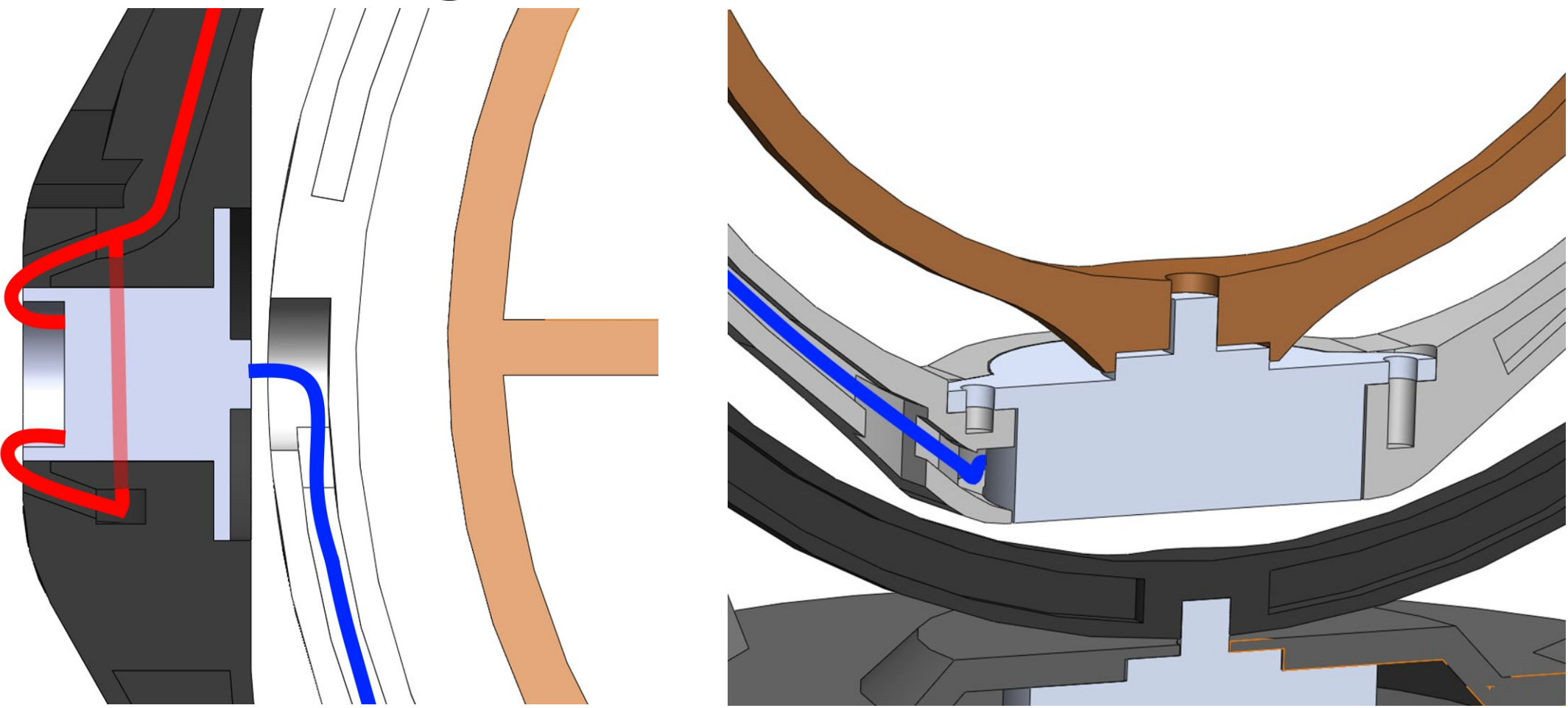
Cross Sections. Left : middle to outer slip ring Right : motor interface between middle and inner ring
